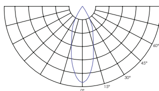
Glass cover 36°
